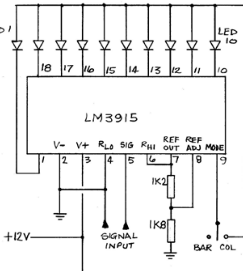
Figure 1 - LM3915N Bar Display Driver
