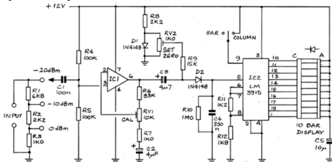
Figure 4 - Circuit diagram
