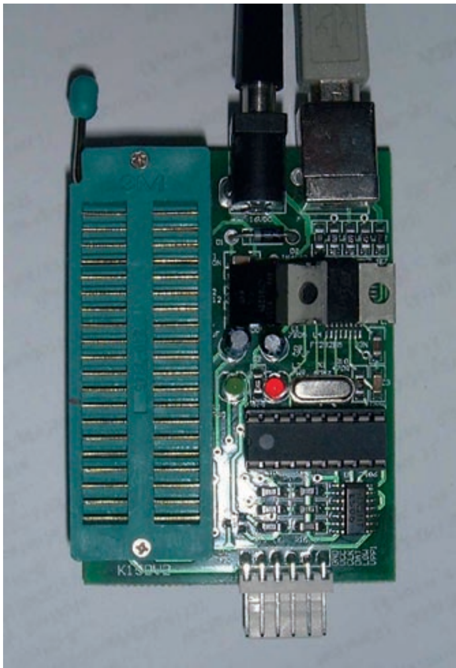
The Quasar Electronics 3150 chip programmer. It can program chips smaller than the 40-pins of the ZIF socket. The connections at the top are for power and USB. The pins at the bottom can be used to program chips which are already mounted on a PCB so they don't have to be removed and placed in the ZIF socket. This is called 'in circuit serial programming'.
